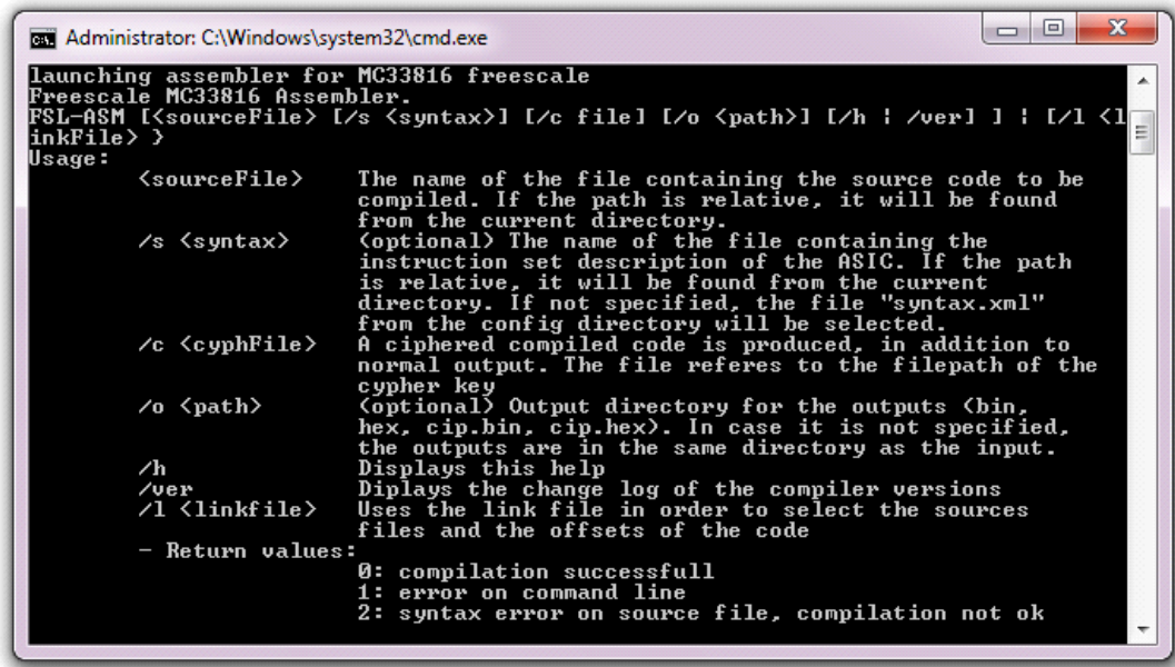
Figure 2. MC33816 Assembler Help Menu
