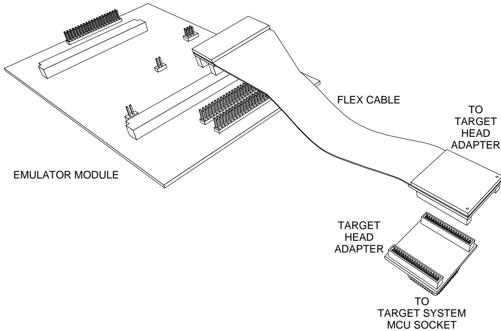
Figure 1: Modular Cable Structure
