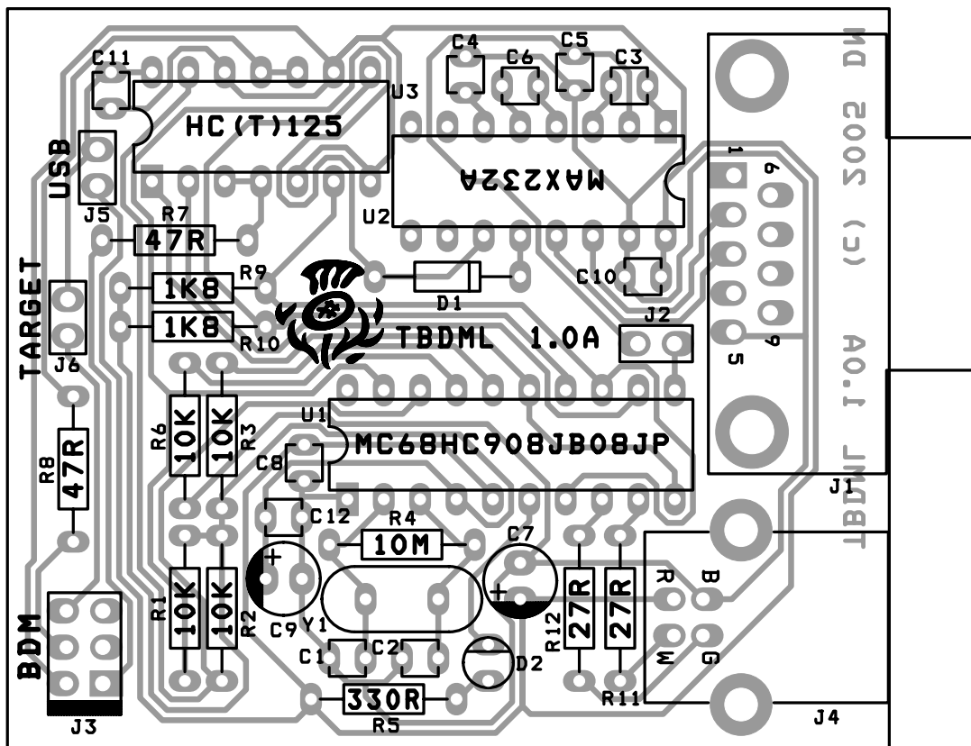
FIGURE 2. TBDML PCB
