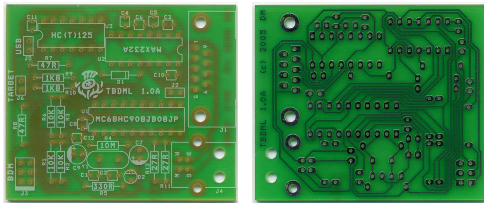
FIGURE 3. TBDML PCB
