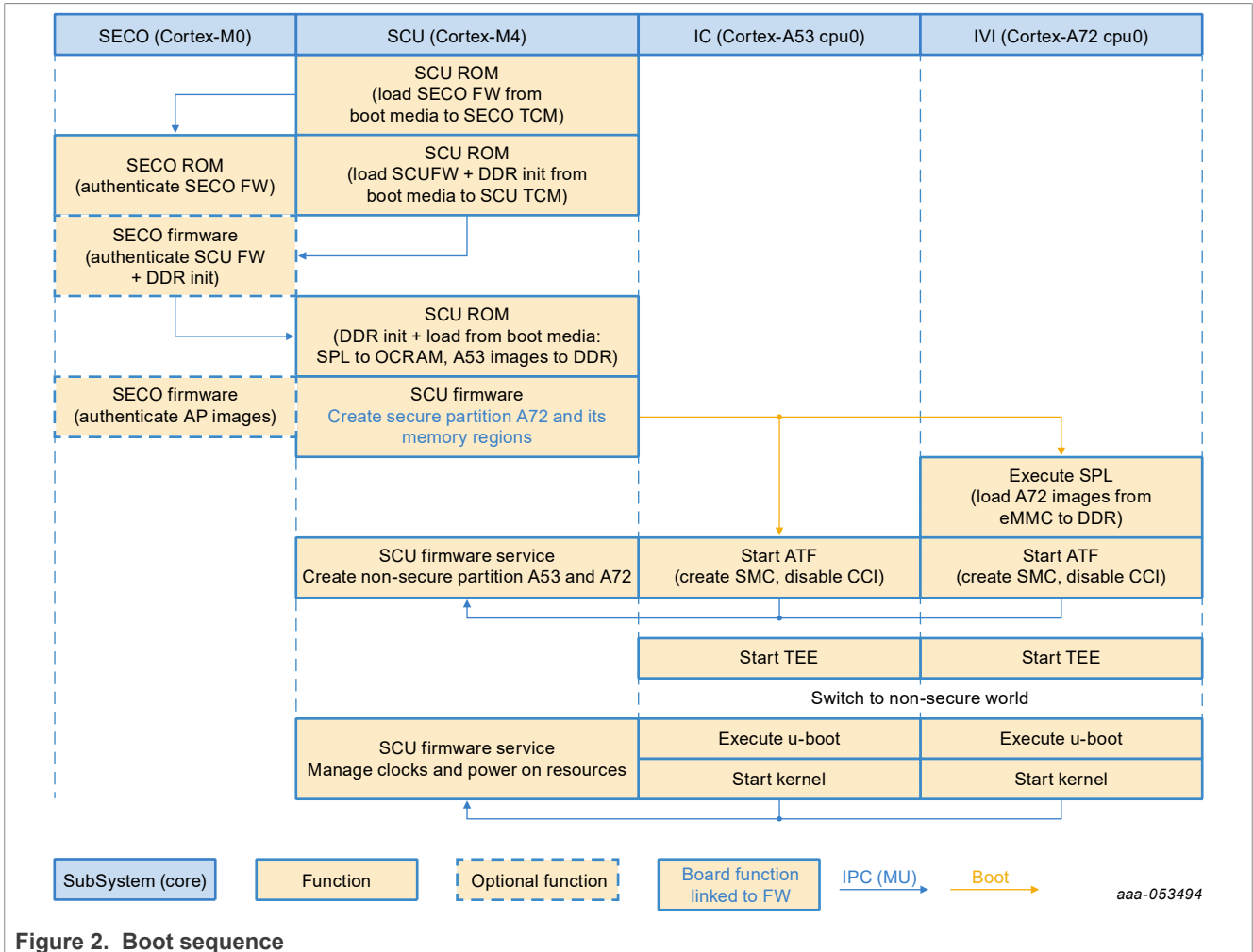
Figure 2. Boot sequence
