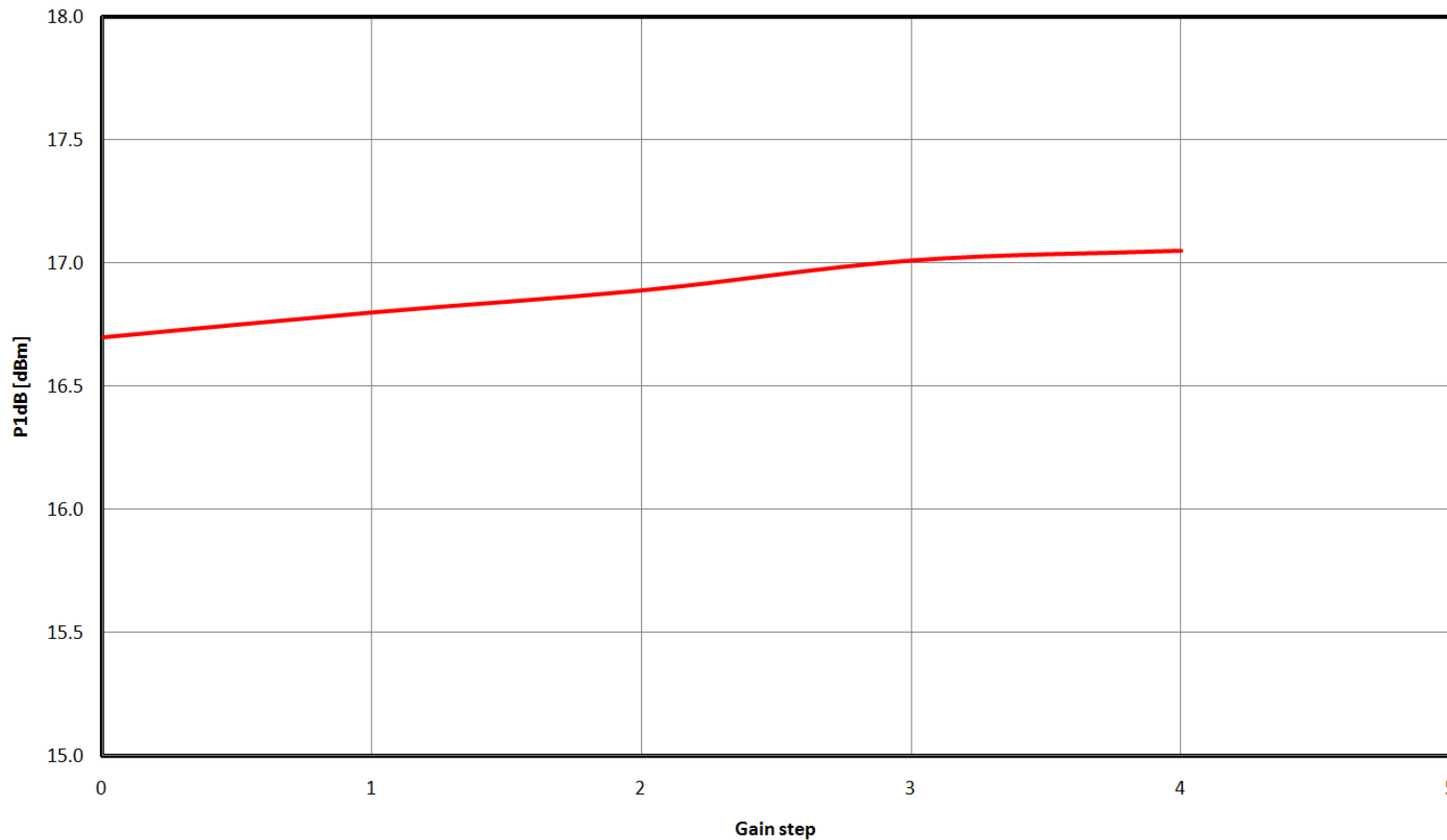
P1dB over the first 5 gain steps Freq=150 MHz
