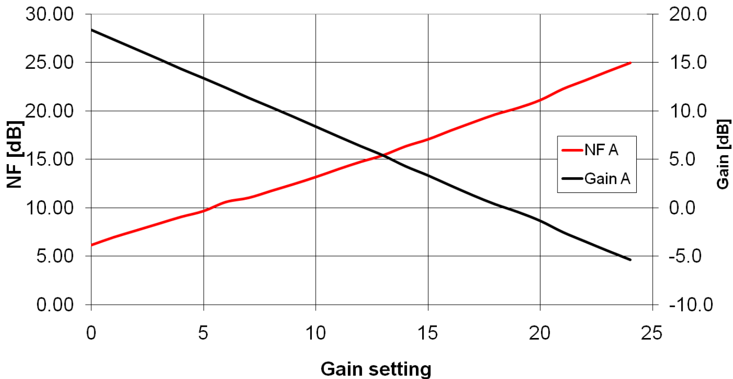
Noise Figure vs Gain settings Freq=150 MHz
