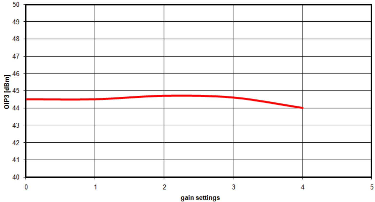
OIP3 over the first five gain settings
