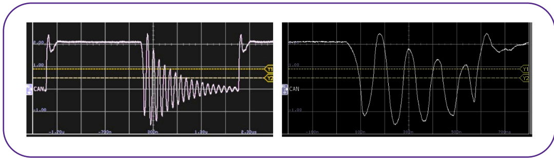
Figure 1: Signal ringing examples at 500kbps (left) and 2Mbps (right). The horizontal lines show the minimum and maximum receiver thresholds. To guarantee reliable communication, the signal must be stable underneath the minimum receiver threshold by the sample point, typically around 70-80% of the bit time. In the 2Mbps example, the signal still peaks above this limit, preventing reliable communication to occur.
