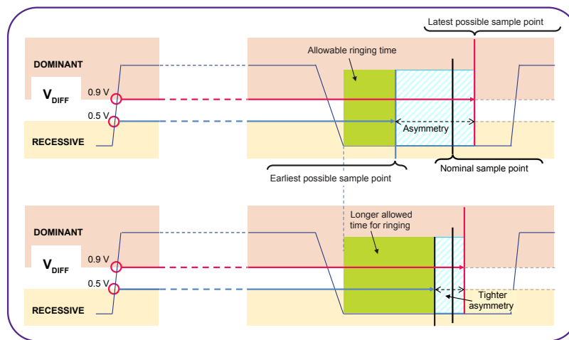
Figure 2: A reduced asymmetry a smaller deviation on when a sample point may occur, which means the earliest possible sample point is later. In turn, this means more time for ringing to occur without affecting network communication.
