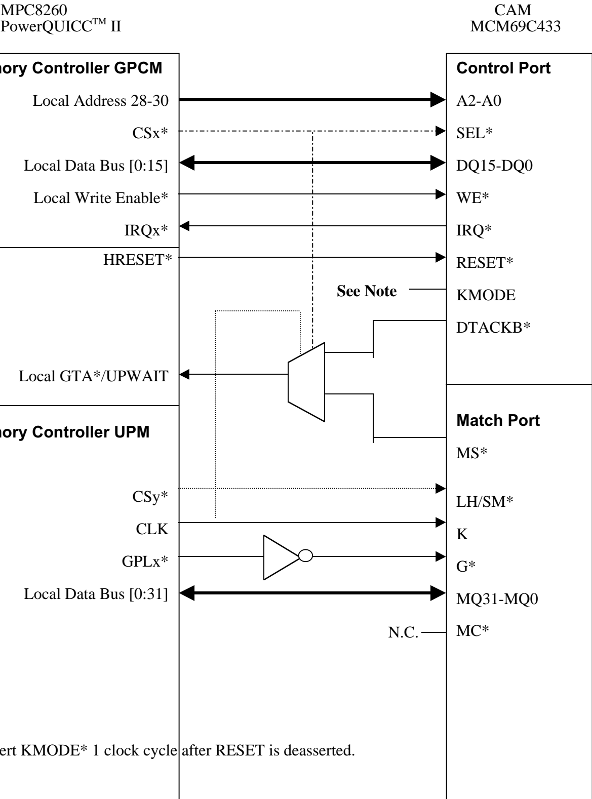
Figure 1: MPC8260/CAM Interface
