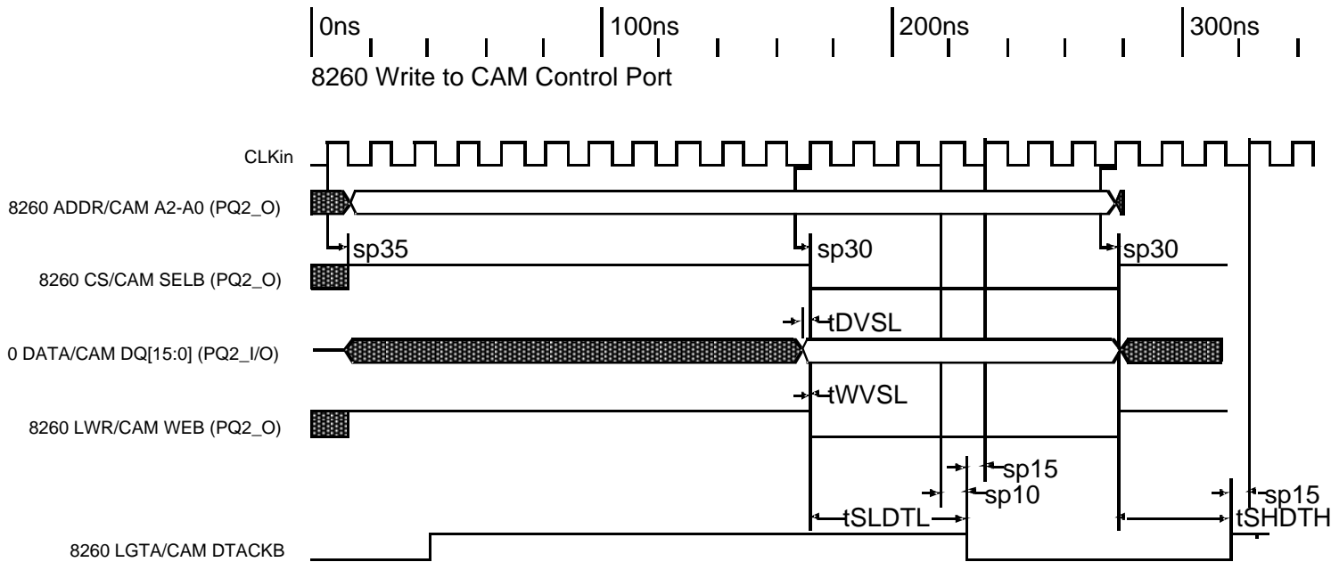
Figure 2: PowerQUICC II™ Write Cycle (CAM Control Port Read)
