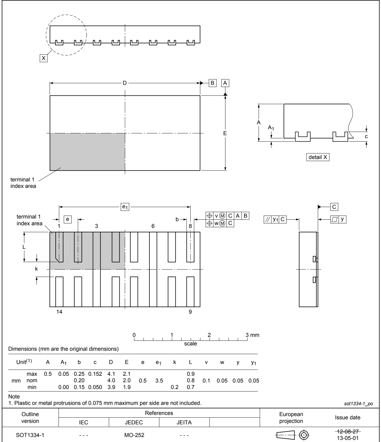
Fig. 1. Package outline DFN4020-14 (SOT1334-1)
