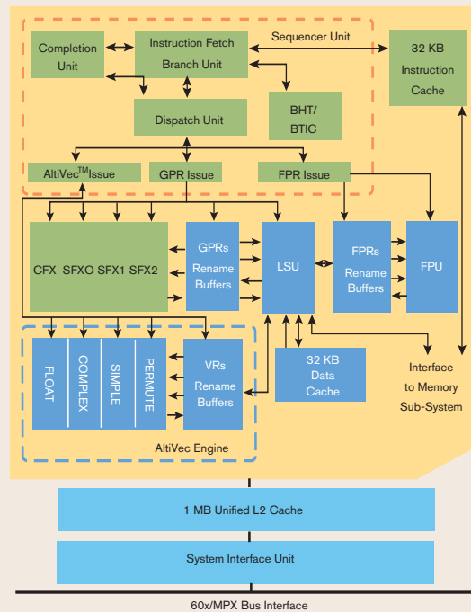
MPC7448 POWERPC® PROCESSOR BLOCK DIAGRAM
