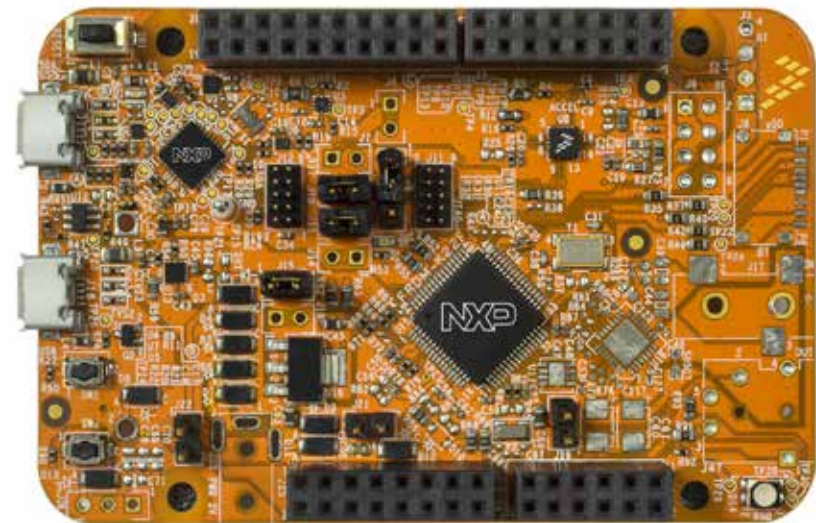
FRDM-K22F
