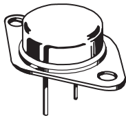
CASE 1, 3, 11 TO-204AA (TO-3)
